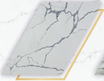
QUARTZ
